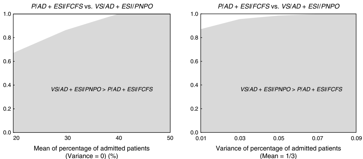
Figure 10. Sensitivity of virtual streaming (VS) and pooling (P) designs with respect to mean \mu_\alpha (left) and variance \sigma_\alpha^2 (right) of the percentage of A patients.
