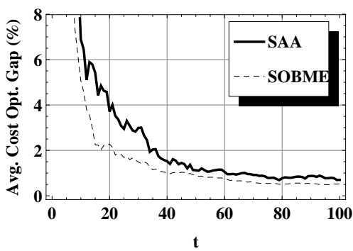
(e) Case II-A-No Bounds
