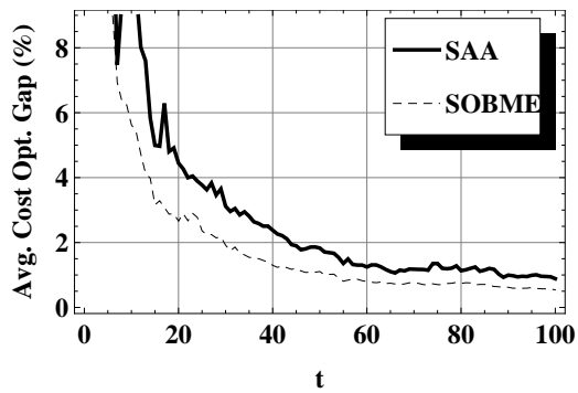
(a) Case I-A-No Bounds
