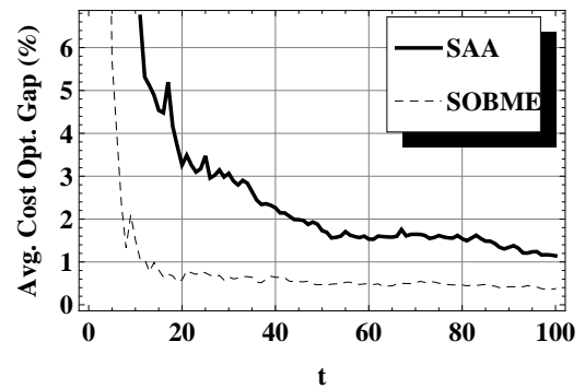
(b) Case I-A-Tight Bounds
