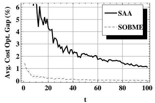
(h) Case II-B-Tight Bounds
