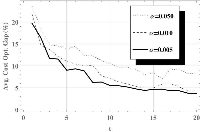
Figure 5 Performance of SOBME under the KMM criteria (Case I-A-No Bounds).
