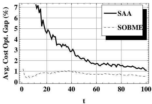
(c) Case I-B-No Bounds
