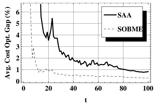
(f) Case II-A-Tight Bounds
