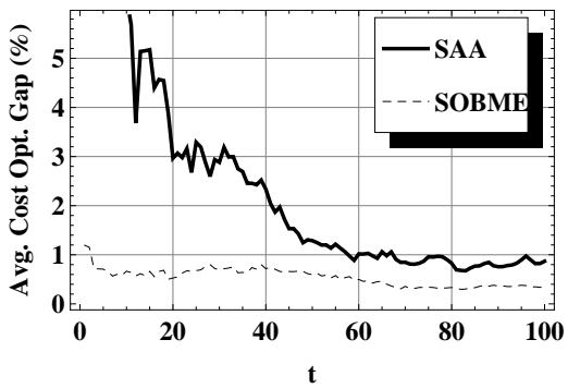
(g) Case II-B-No Bounds
