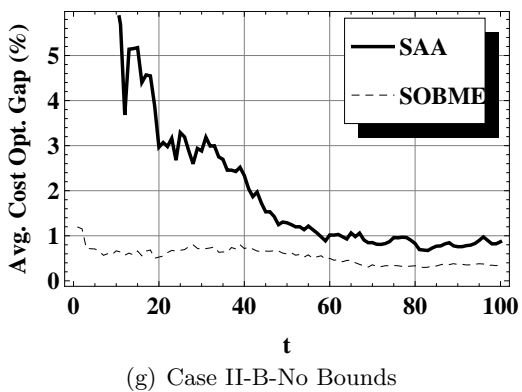
Figure 1 Comparison of SAA and SOBME under various cases.
