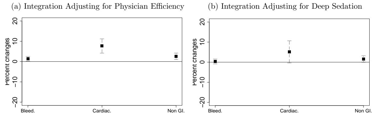
Figure 3: DID Estimates: Mediation Analyses
