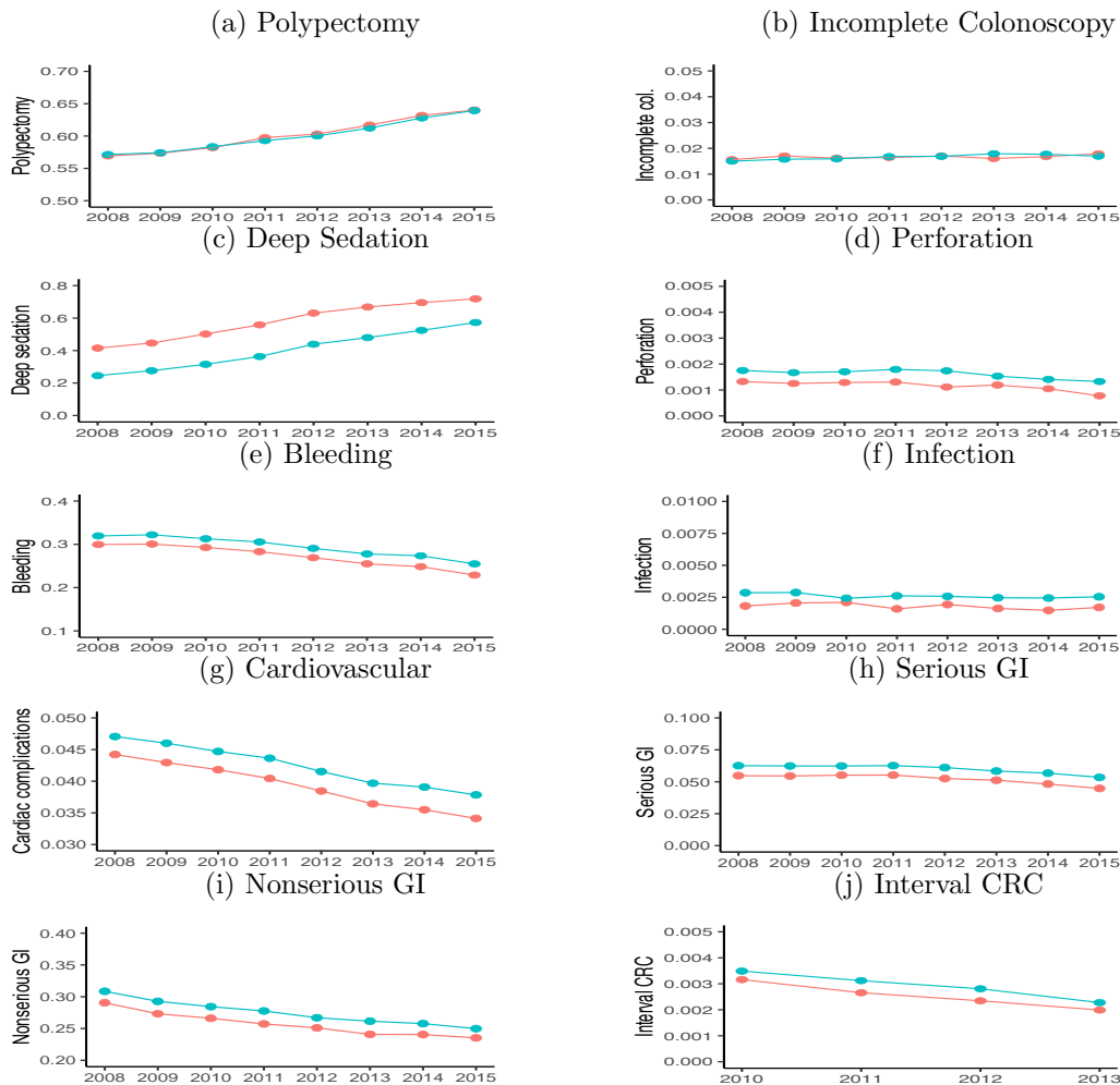
Figure EC2: Trends of Process Measures and Post-Procedure Complications
