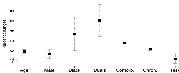
Figure EC3: Average Effect of Integration on Patient Composition, Scaled into Percent Changes
