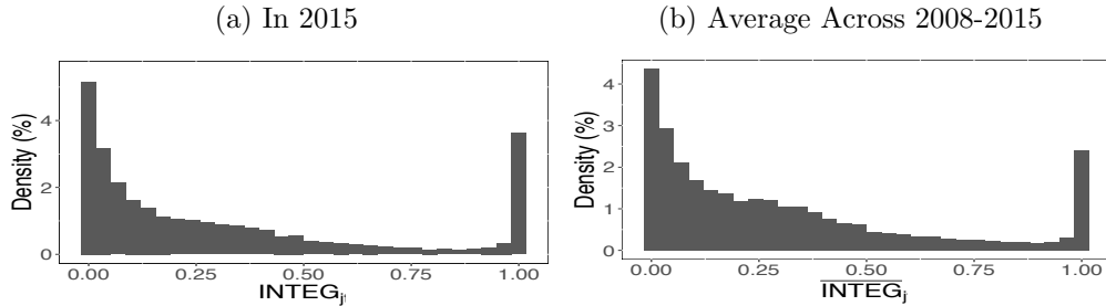
Figure EC1: Distribution of INTEG_{jt}
