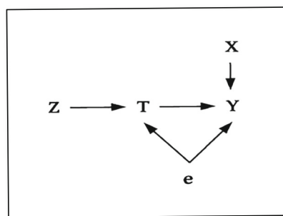
Fig. 6 The Directed Acyclic Graph (DAG) Behind Our Instrumental Variable Approach [ Z : generalist is assigned; T : assignment matches the guideline; Y : outcome variable (30-day readmissions); X : vector of control variables]
