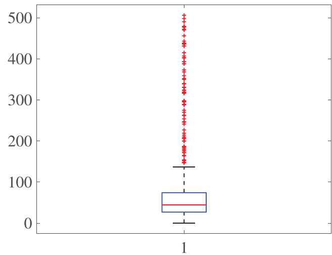
FIGURE 1 Boxplot for scheduling delays [Color figure can be viewed at wileyonlinelibrary.com]
