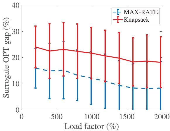
FIGURE 4 The effect of multiple visits on the surrogate OPT gap [Color figure can be viewed at wileyonlinelibrary.com ]
