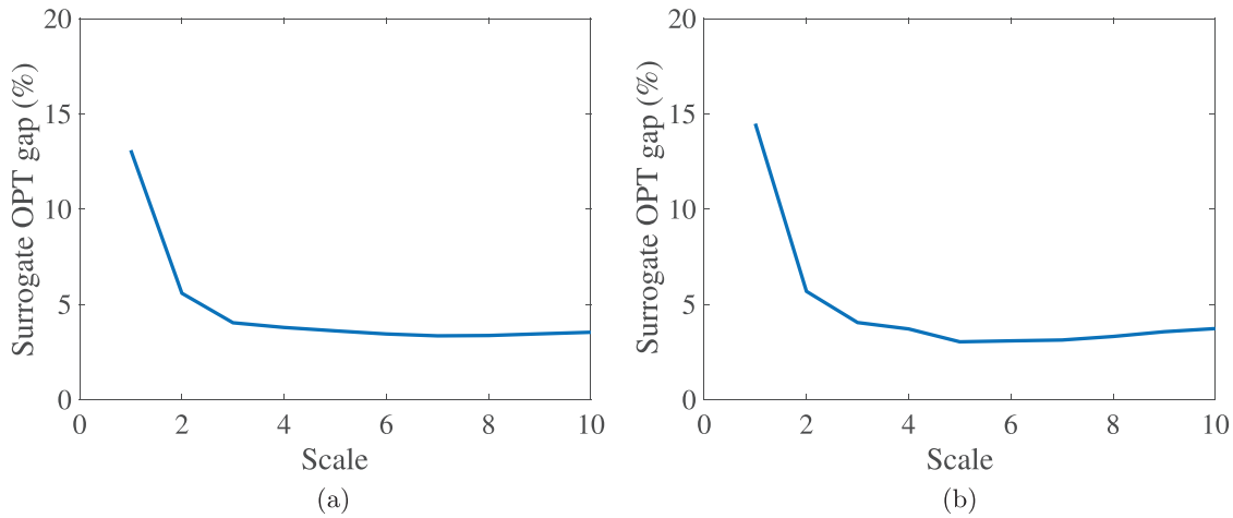
FIGURE 2 Surrogate OPT gaps on the scaled data set. (a) Surrogate OPT gap with K = 4 clusters. (b) Surrogate OPT gap with K = 5 clusters [Color figure can be viewed at wileyonlinelibrary.com]
